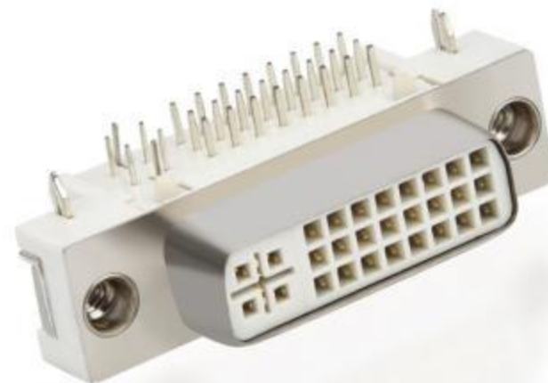
DVI 24+5 Female
